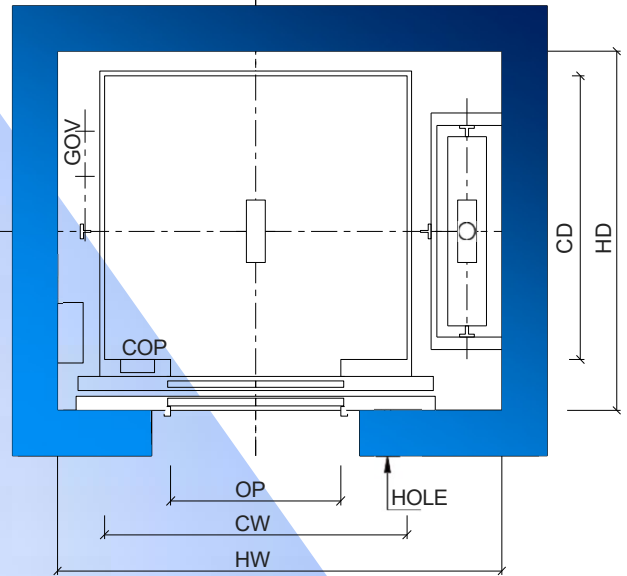
HOISTWAY PLAN
